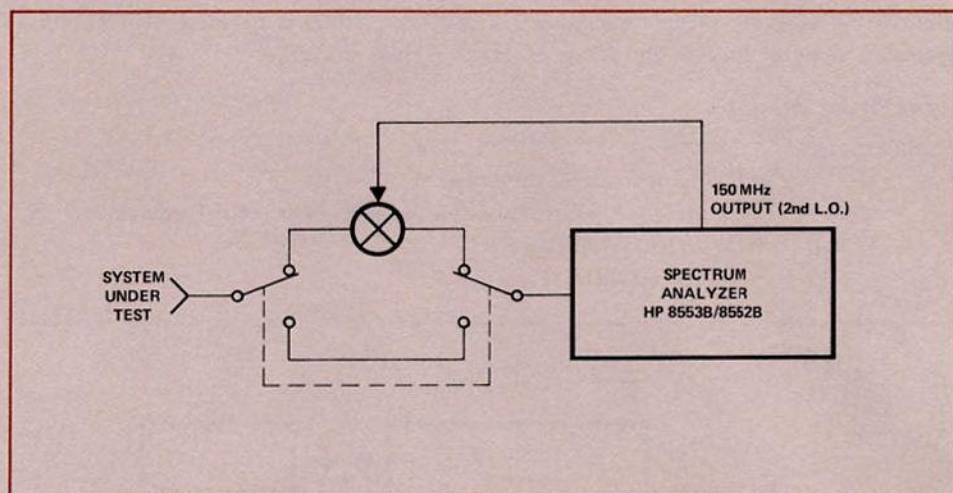
Figure 5.3 Another Method for Hum Measurement (Preferred Accuracy)
